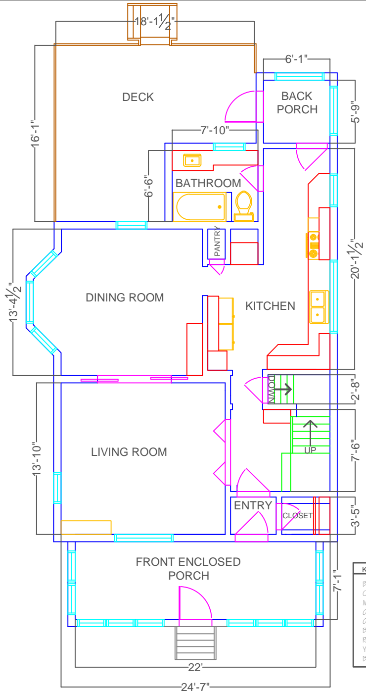
217 EAST STREET LEVEL 1
